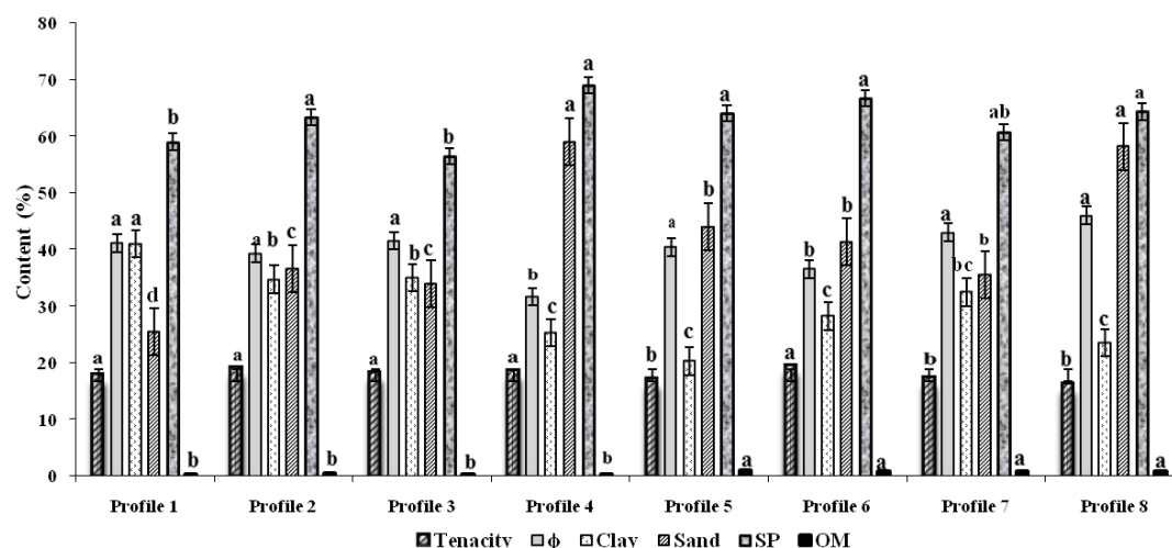
Fig. 4. Mean compression of some soil properties in different soil profiles. ( \phi : Internal friction angle; SP: Saturation percentage; OM: Organic matter).
