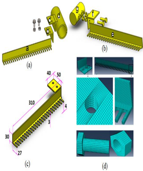
Fig. 4. (a) OSS components; (b) ISS components; (c) Shoulder dimension in millimeter; (d) Shoulder components mesh.
