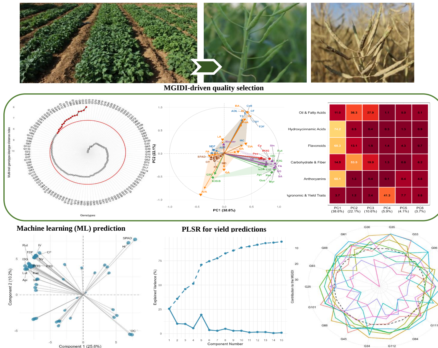
Fig. 6. A schematic overview of the integrated analytical framework combining dynamic metabolic profiling, multi-trait selection, and machine learning prediction for drought-resilient rapeseed breeding. The workflow includes time-resolved metabolic profiling of 119 genotypes at 20 and 40 DAP using FT-NIR spectroscopy and HPLC-DAD; MGIDI-driven quality selection identifying elite genotypes balancing yield, drought resilience, and nutritional quality; and PLSR and machine learning models achieving high predictive accuracy for seed yield, with SPAD as the dominant predictor
