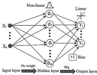
Fig. 2. Diagram of RBF-NN architecture.
