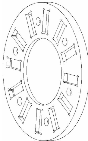
Fig. 9. 3D view of non-ferromagnetic holder
