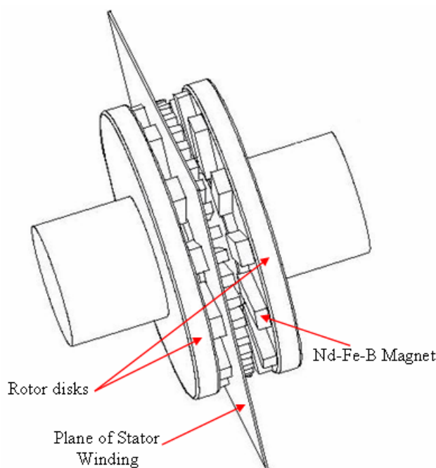
Fig. 1. The structure of the axial flux machine
