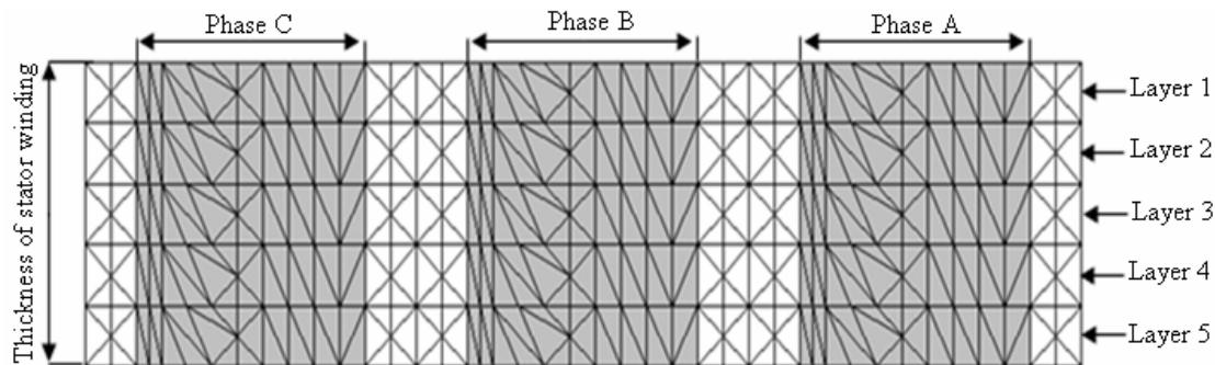
Fig. 6. Schematic of meshed winding and its layers
