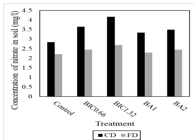
Fig. 5. Average nitrate concentration in soil (mg/L). CD: control drainage, FD: free drainage, BIC0.66: biochar 0.66%, BIC1.32: biochar 1.32%, BA1: bagasse 1%, and BA2: bagasse 2%.
