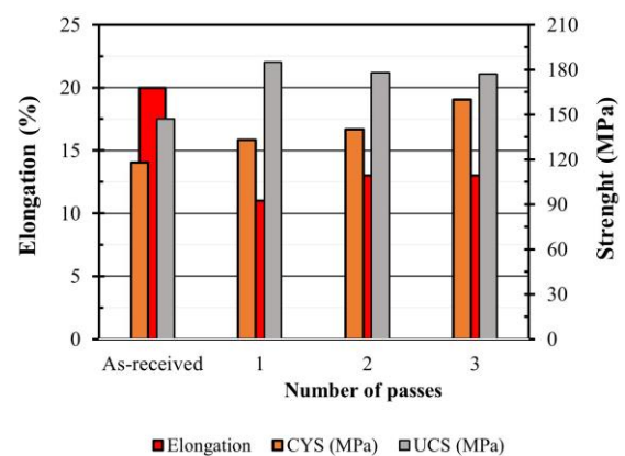
Fig. 9. Diagrams of ultimate tensile strength (UCS), yield strength (CYS), and elongation for the as-received sample and CGPed Al-1050 after different numbers of passes.
