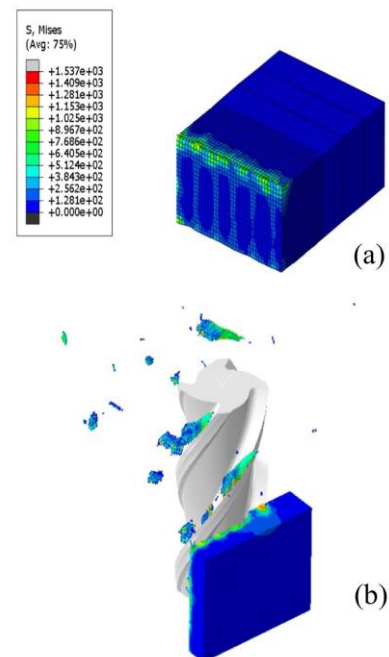
Fig. 6. (a) The residual stress caused by milling and (b) the method of chip removal in the simulation.
