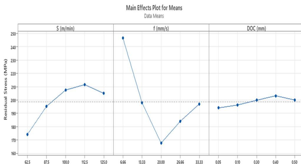
Fig. 7. The effect of milling parameters on residual stress.
