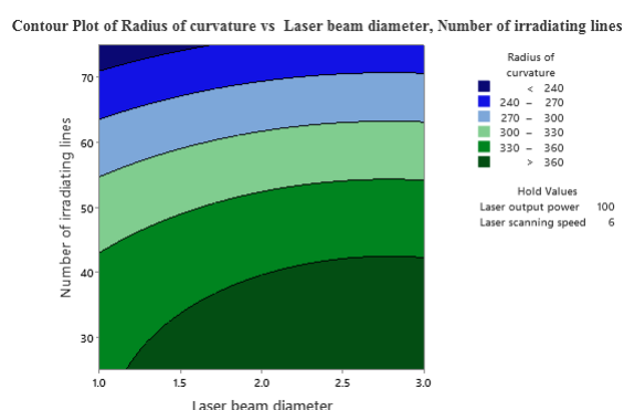
Fig. 7. Interaction between LBD and NIL and their effect on the RC of tube.
