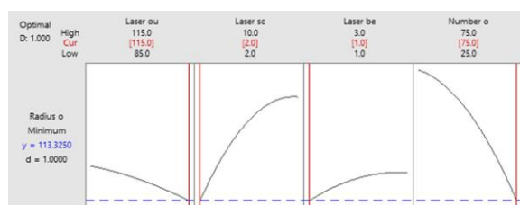
Fig. 8. Optimal conditions of input parameters to achieve the minimum RC value of the tube.
