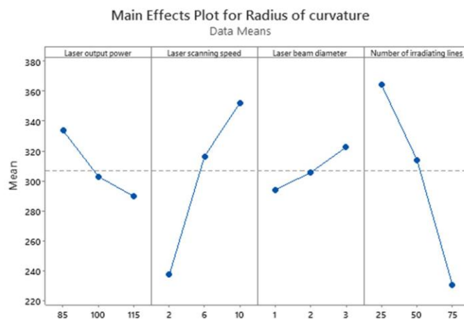
Fig. 4. The effects of input parameters on RC of deformed tubes.
