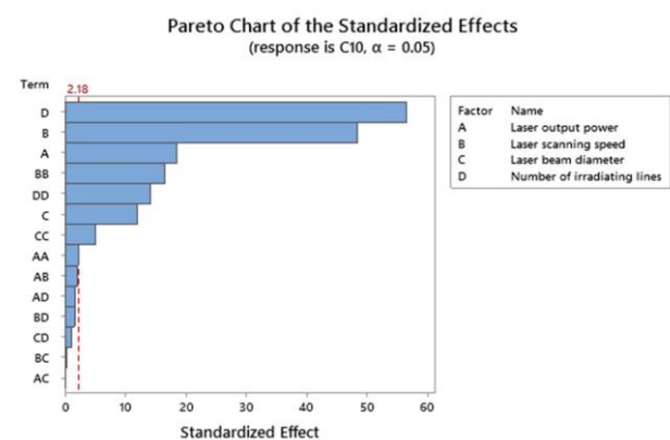
Fig. 2. Pareto diagram plotted based of the analysis of RC.
