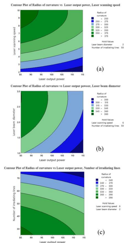
Fig. 5. Interactions between LOP and other input parameters and their effects on the RC of tube: (a) LOP - LSS, (b) LOP - LBD, and (c) LOP - NIL.
