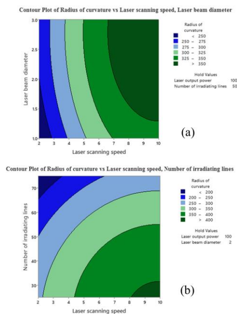
Fig. 6. Interactions between LSS and other parameters and their effects on the RC of the tube: (a) LSS - LBD, (b) LSS – NIL.
