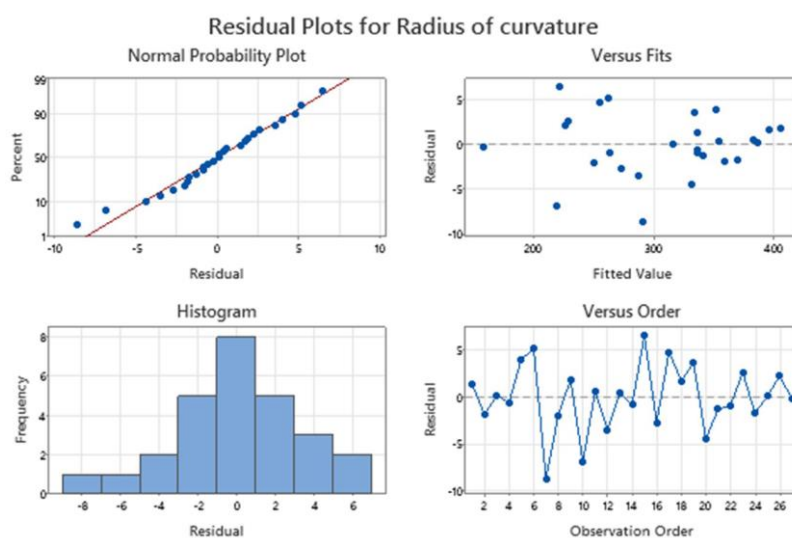
Fig. 3. Residual plots of the employed model in the laser tube forming process.
