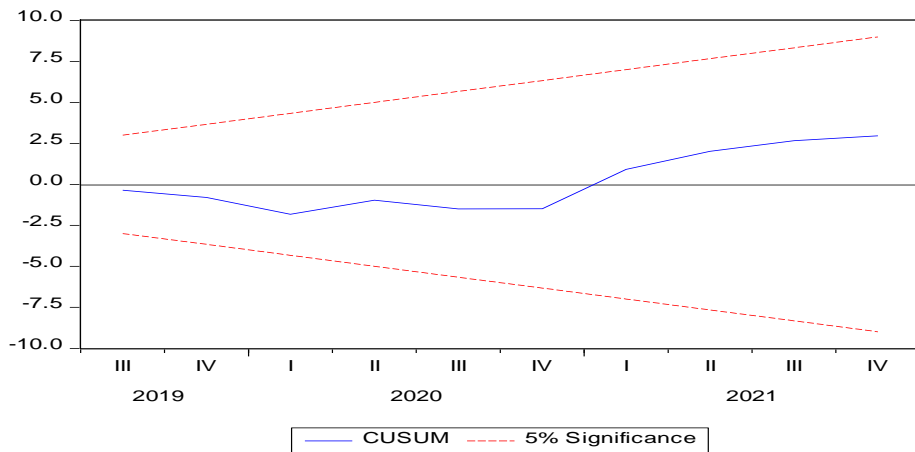
Figure B1. CUSUM Test
