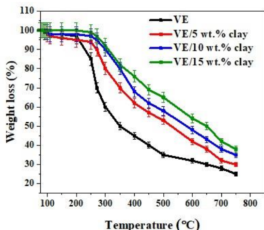
Fig. 7. TGA curves of VE/clay composites with varying clay contents.
