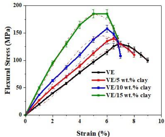
Fig. 4. Flexural stress-strain curves of VE/clay composites with varying clay content.
