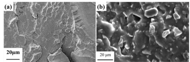
Fig. 3. Fracture surfaces of (a) pristine VE and (b) VE composite containing 5 wt.% clay after tensile testing.
