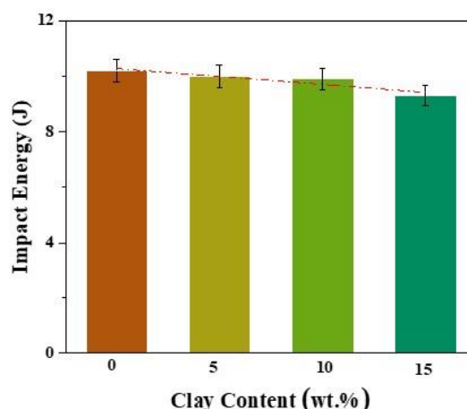
Fig. 5. Comparison of impact energy for VE/clay composites with varying clay content.
