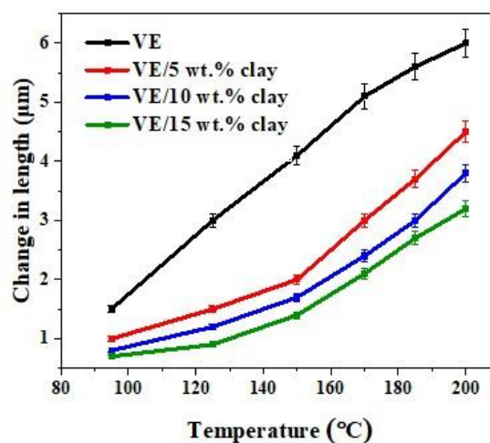
Fig. 6. Temperature-dependent dimensional of VE/clay composites with varying clay content.
