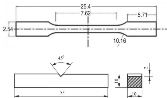
Fig. 1. Shape and dimensions of the standard specimen used for tensile and bending test [15].
