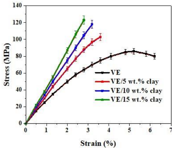
Fig. 2. Stress-strain curves of VE/clay composites with varying clay content.
