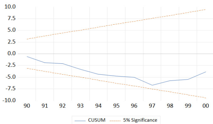
Figure 1. CUSUM Test for Cumulative Sum of Recursive Residuals
