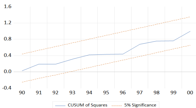
Figure 2. CUSUMSQ Test for Cumulative Sum of Squares of Recursive Residuals
