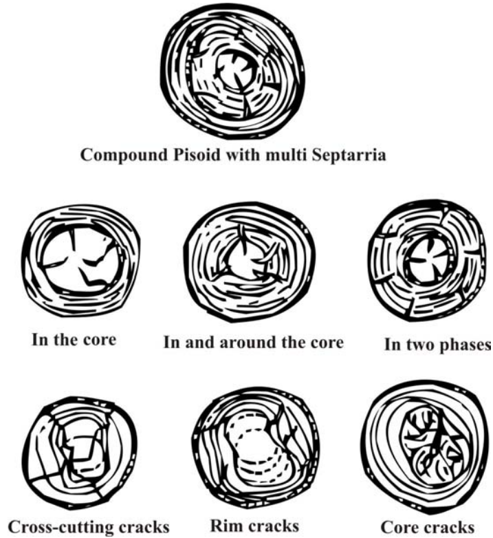
Fig. 17. Schematic representation of some types of septaria observed in lag (after Boulange, 1984)
