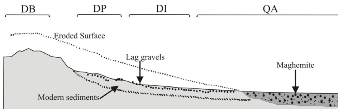
Fig. 3. Schematic classification of landform geomorphological classification units in erosional and depositional environments of surface sediments (after Senior, 1992)
